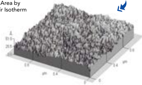
Mesoporous structure
